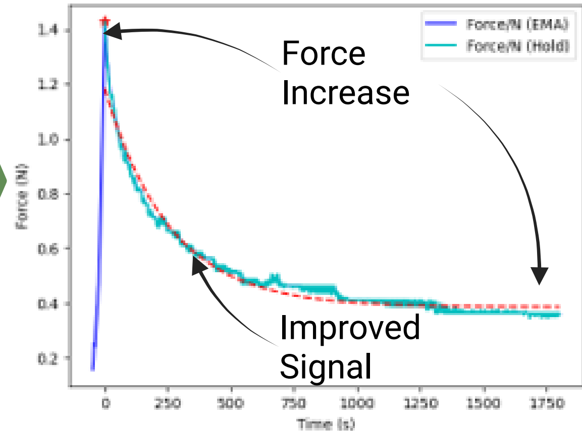
Improved Setup
